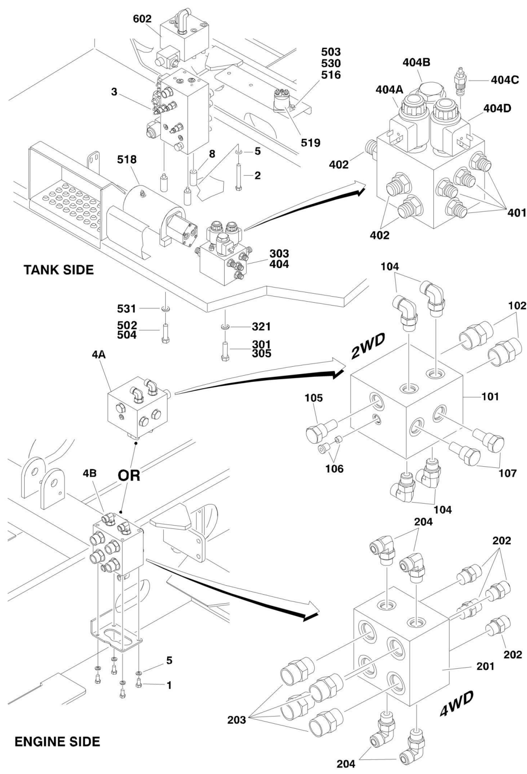
FIGURE 2-1. CONTROL VALVES INSTALLATION
